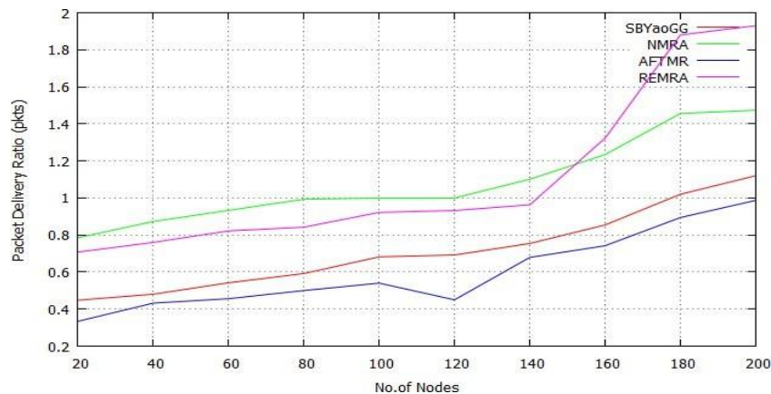
Figure 3: No. of Nodes Vs Packet Delivery Ratio using REMRA Scheme
