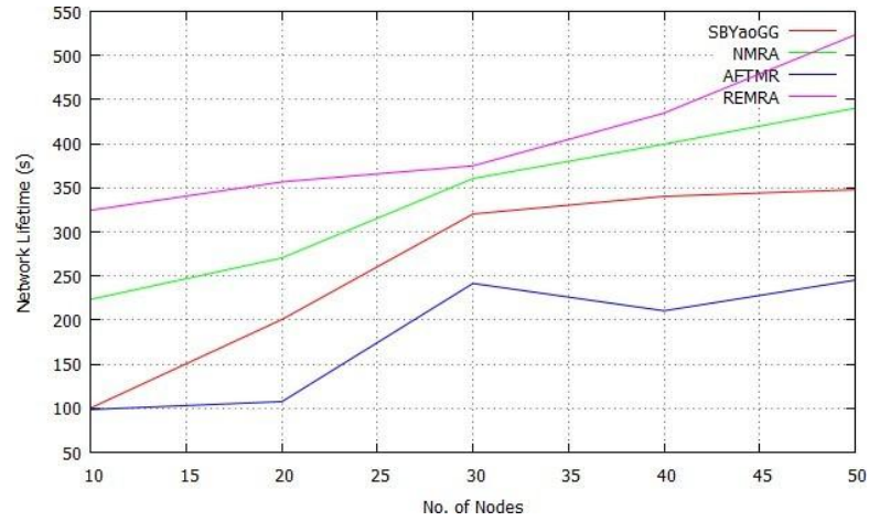
Figure 4: No. of Nodes Vs Network Lifetime using REMRA Scheme
