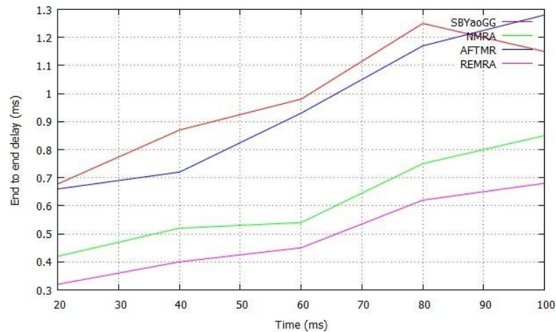
Figure 5: Time Vs End to End Delay using REMRA Scheme
